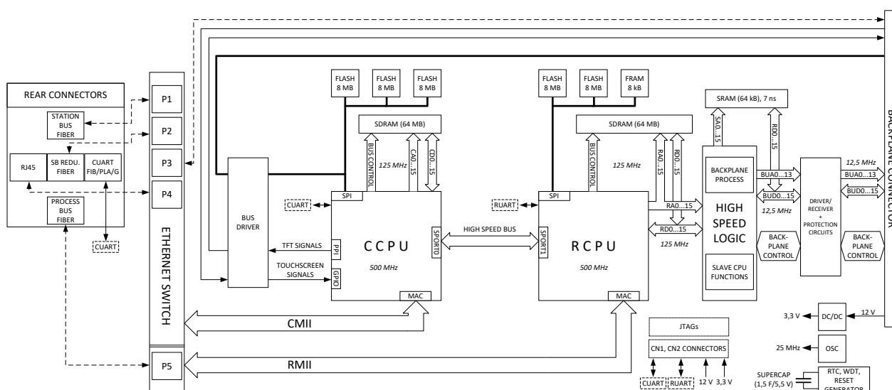
Figure 4-1 CPU block diagram
