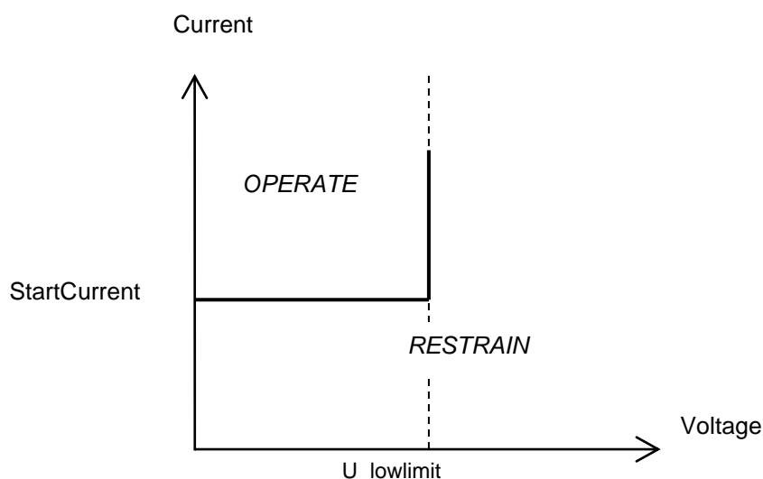
Figure 2-6 Voltage controlled characteristic
