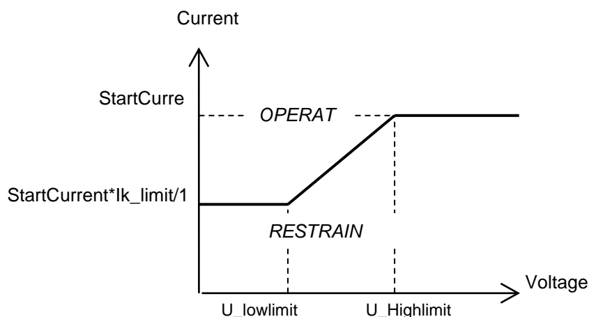
Figure 2-5 Voltage restrained characteristic
