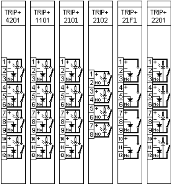
Figure 9-1 Tripping modules
