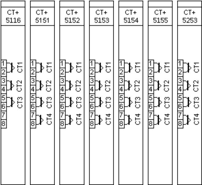
Figure 5-1 CT modules
