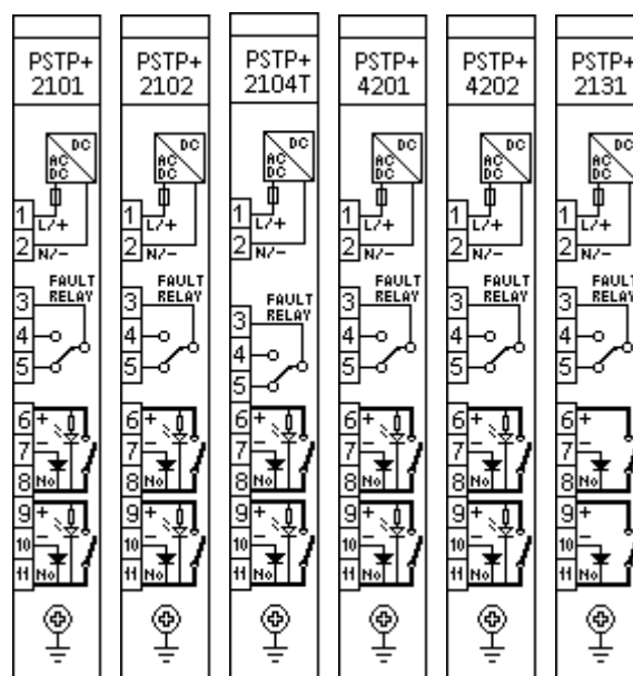
Figure 18-1 Power supply with 2 Ch. TRIP modules
