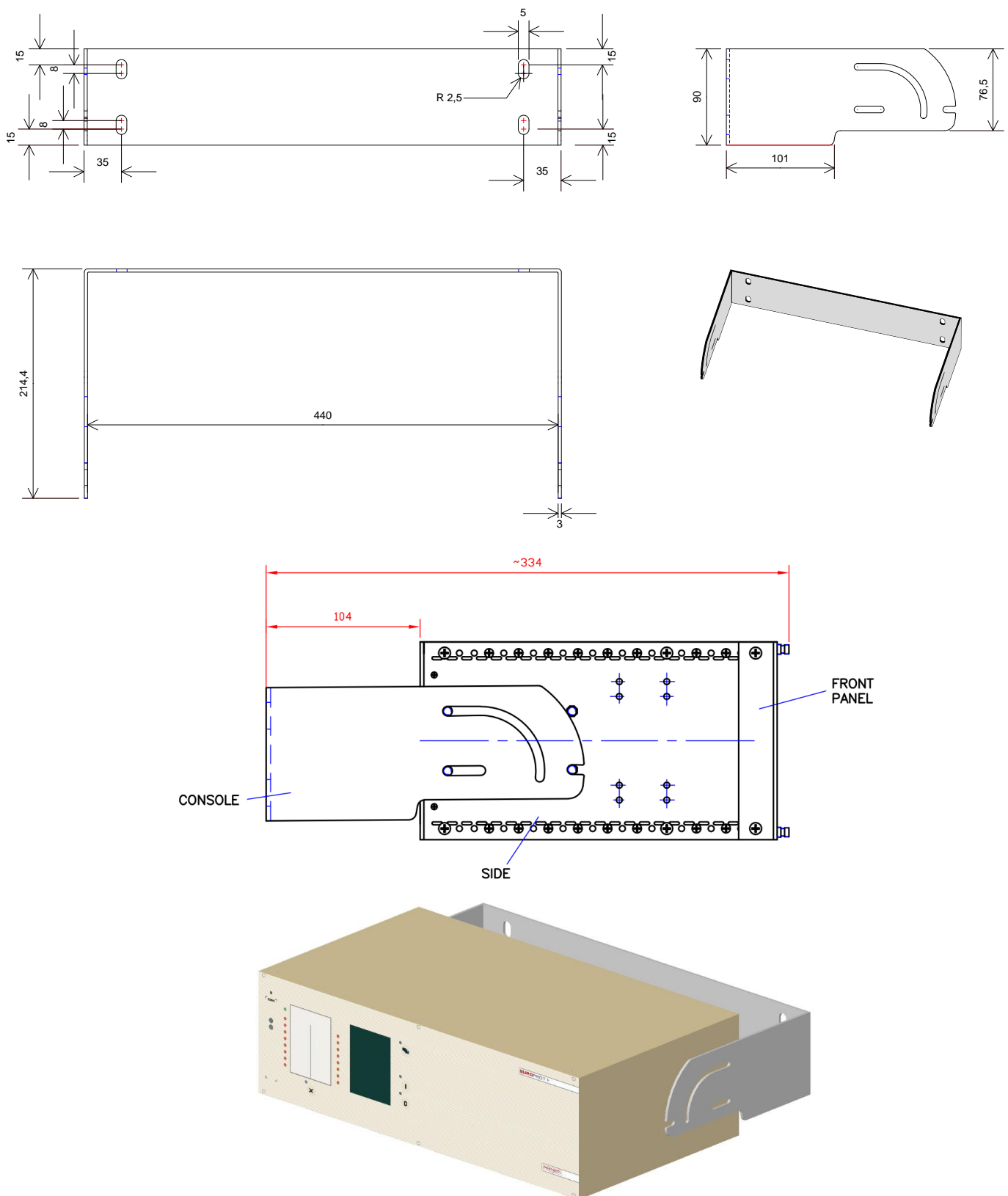
Figure 21-23 84 HP fold-down mounting
