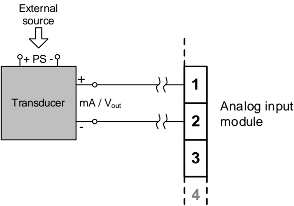
Figure 11-2 AI wiring
