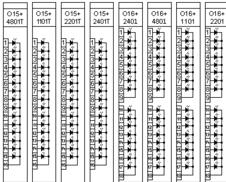
Figure 7-1 Binary input modules
